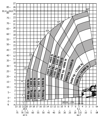
Rotation on lowered stabilizers with forks
