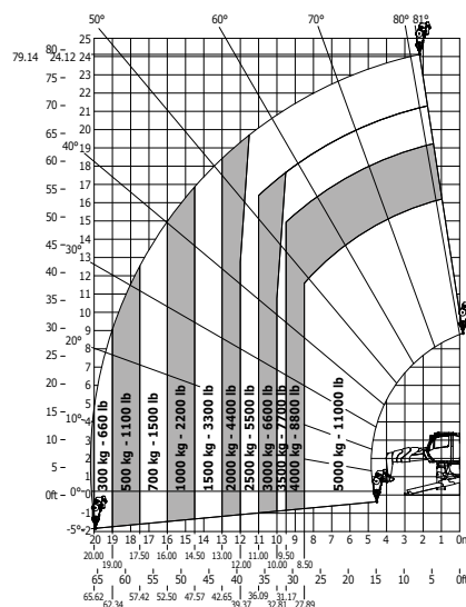
Rotation on lowered stabilizers with 1500 kg jib
