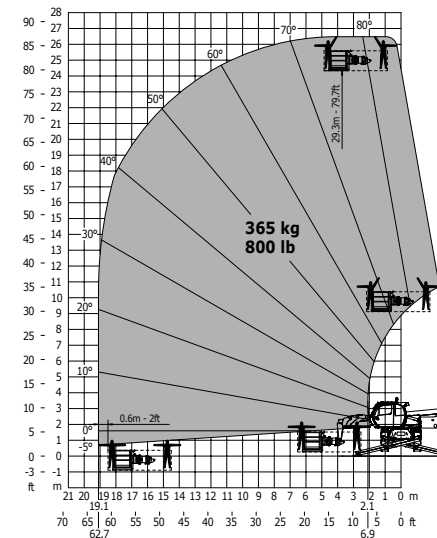
Rotation on lowered stabilizers with 365 kg platform
